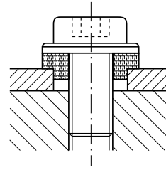
Absorbs expansion and isolates screws under dynamic load.
