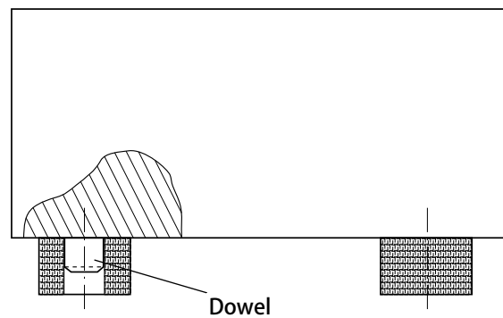
Machine mounted on cushions located on dowels.
