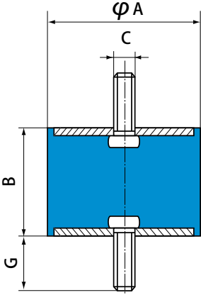
双边螺柱
